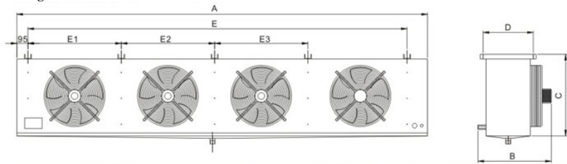
Cooling fan installation dimensions:
